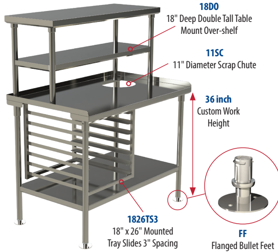
TB312-3048 16 Gauge Stainless Steel Top with 1.5" Backsplash and Open Base and U-Brace
